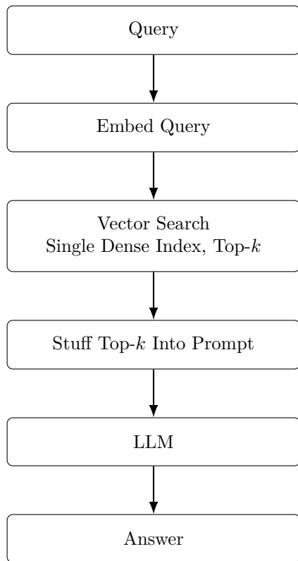
Figure 1: Baseline RAG. One retrieval signal, no ranking beyond raw similarity, no relevance floor, no caching, no tenant awareness, and no validation of any of the above.
