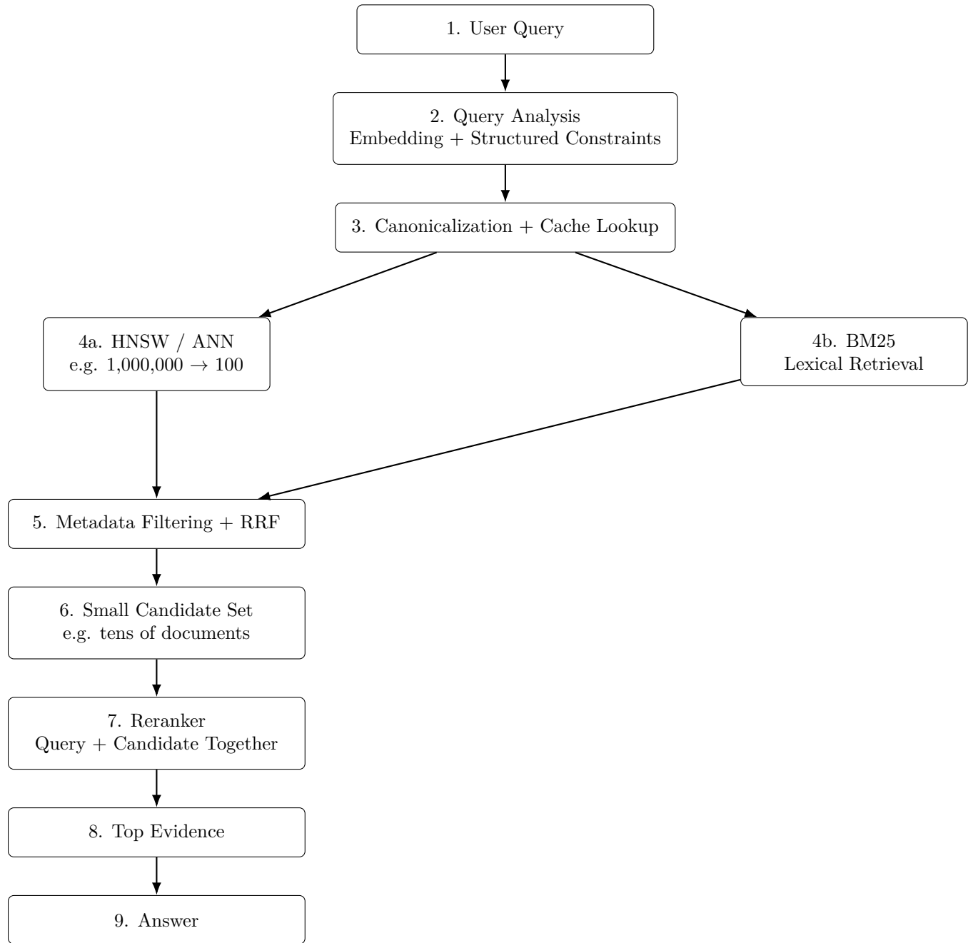
Figure 2: Simplified query workflow. The large document collection is reduced using fast retrieval methods before the expensive reranking stage. HNSW provides semantic candidate retrieval, BM25 provides lexical candidate retrieval, RRF combines the rankings, and the reranker carefully evaluates only the resulting small candidate set.
